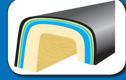
8-10mm Thick, Oven Cured 6 Layer "Tough Bond" Shell
